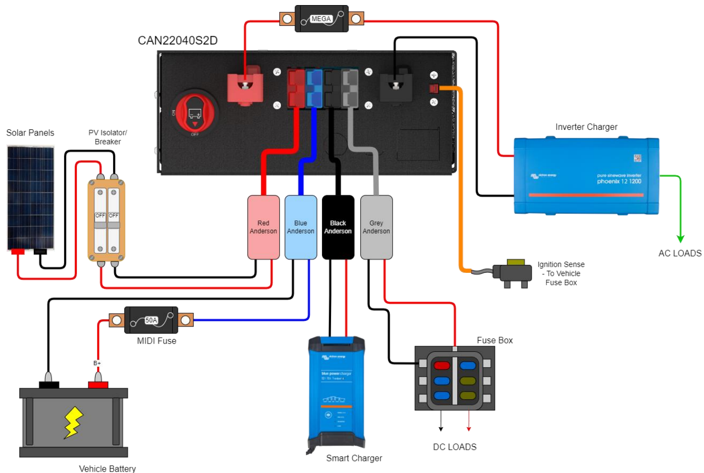
Figure 4 Example Use Case of CAN22040S2D Power Hub
