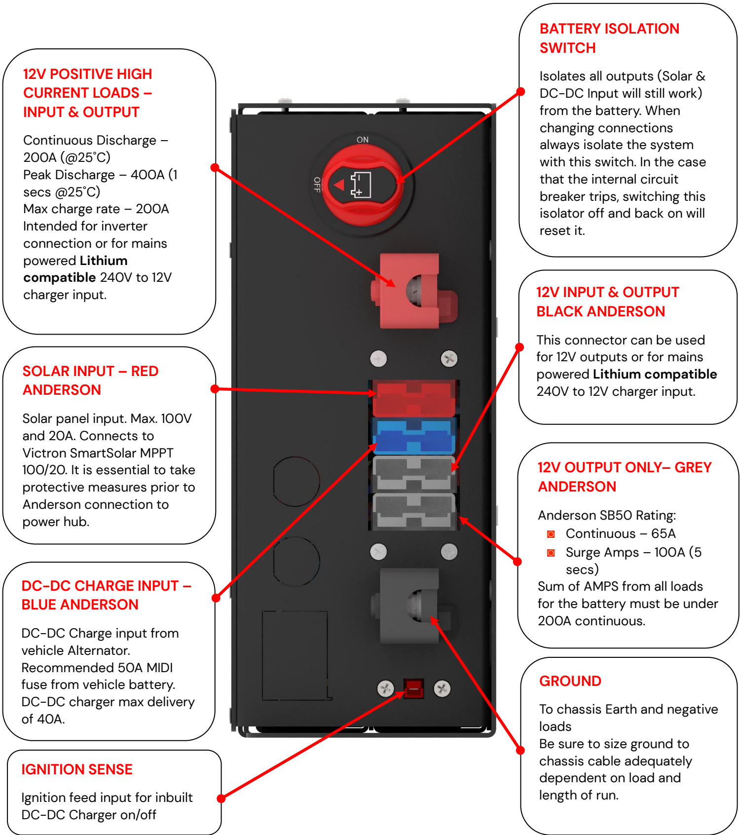
Figure 1 CAN22040S2D Power Hub Connection Description
