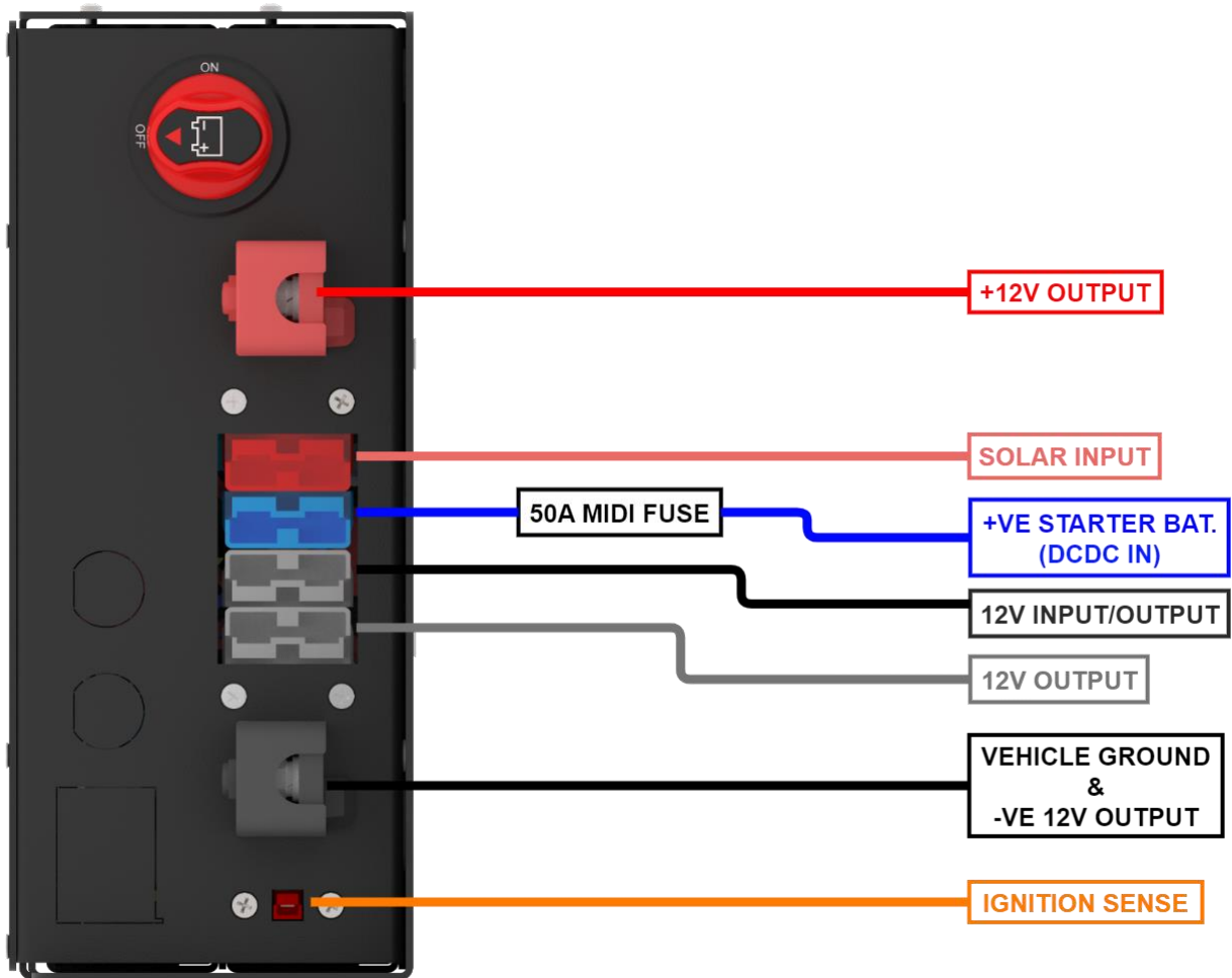
Figure 3 CAN22040S2D Power Hub Example Wiring Schematic
