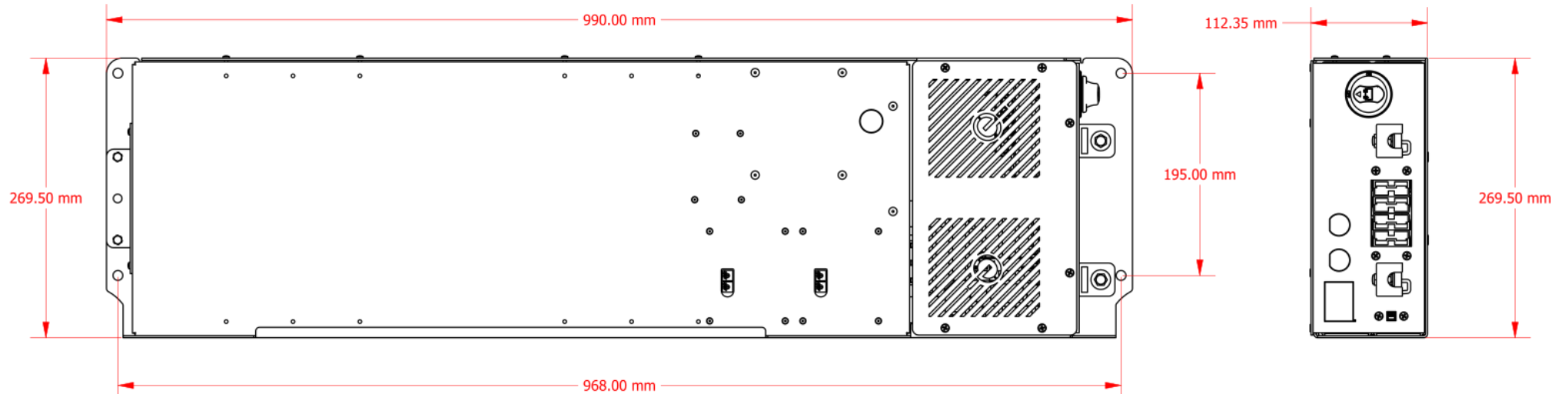
Figure 2 CAN22040S2D Power Hub Dimensions
