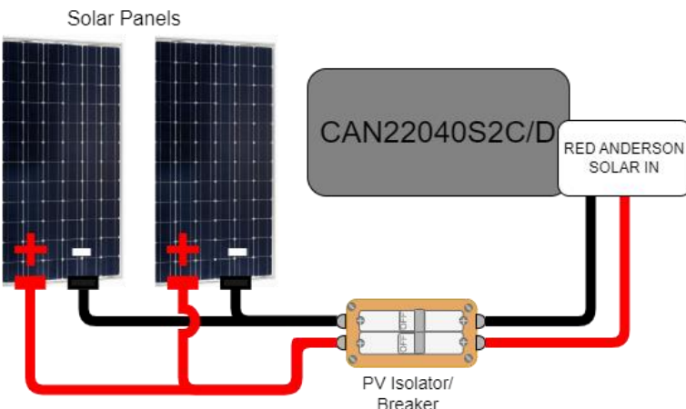
Figure 9 Example Parallel Configuration of Solar Panel Array
