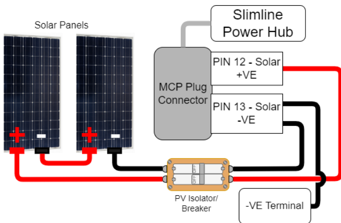
Figure 8 Example Series Configuration of Solar Panel Array
