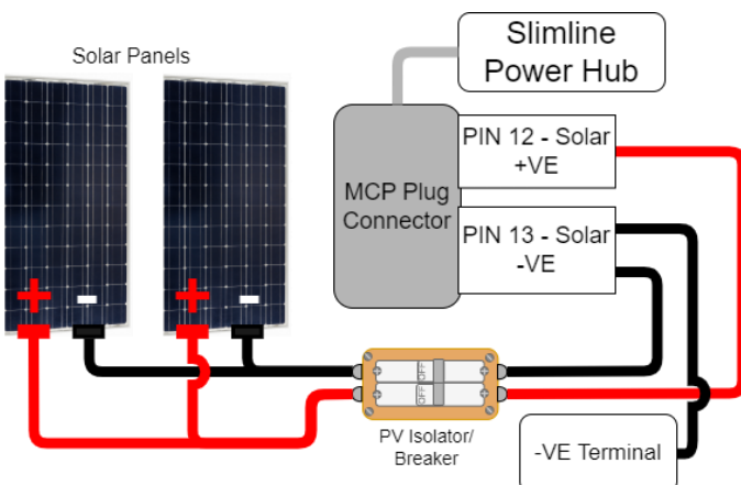
Figure 9 Example Parallel Configuration of Solar Panel Array
