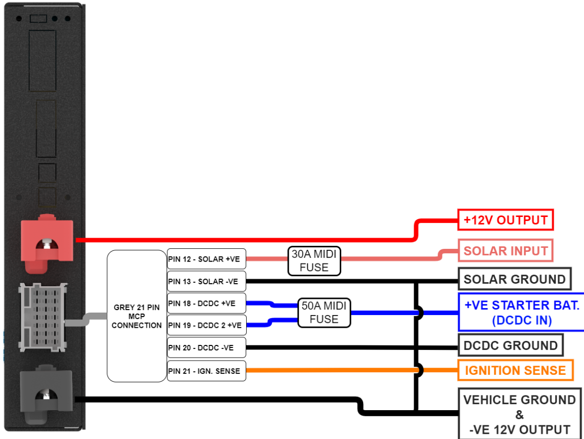
Figure 4 CANL110NO40S15SH Slimline Mini Hub Example Wiring Schematic
